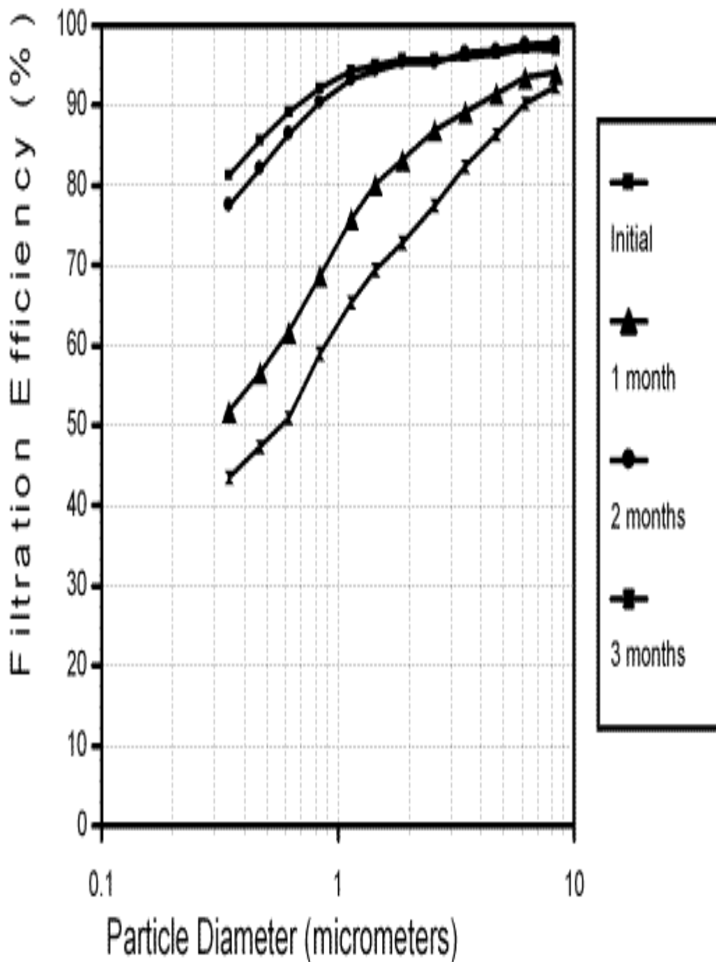
Figure 1. Real-life ESP efficiency curves before and after in-home operation for 1, 2 and 3 months.
